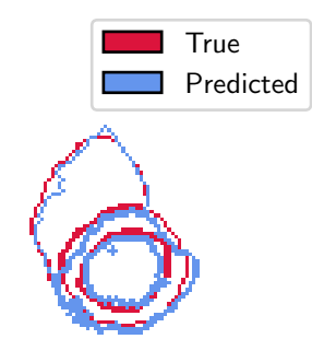
segmentations
